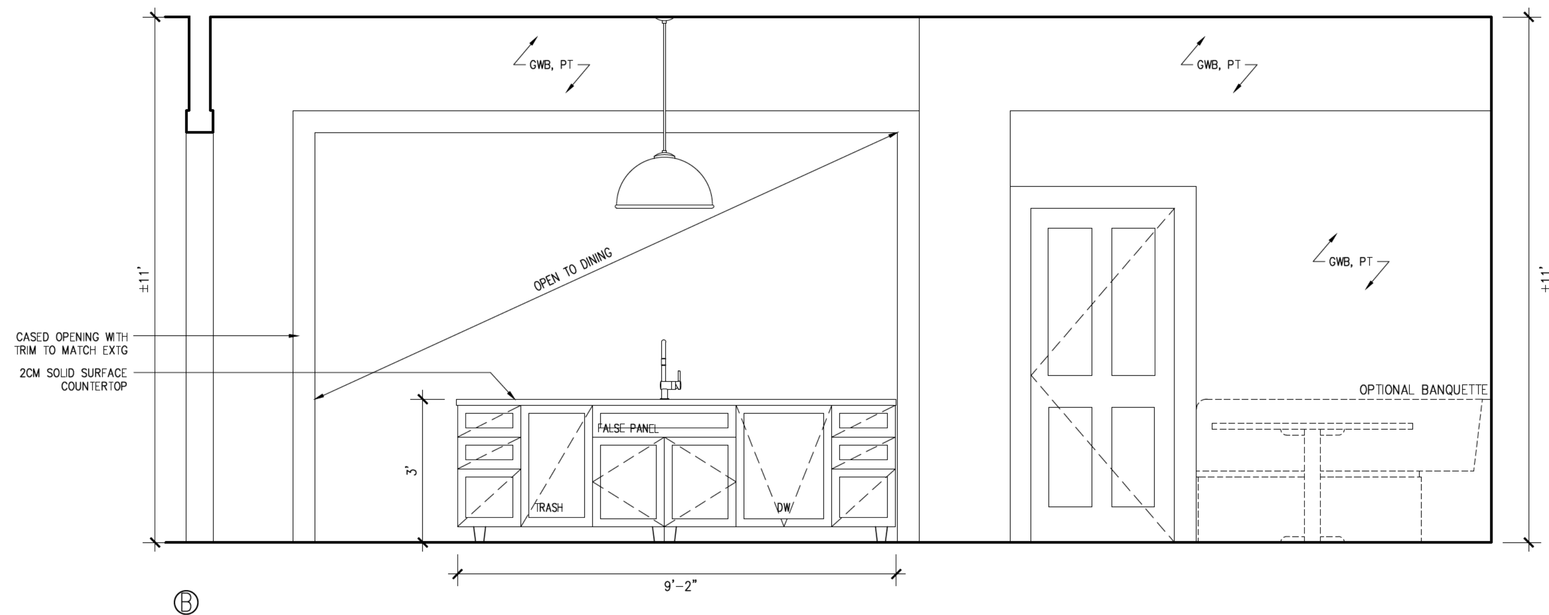
2 INTERIOR ELEVATION: KITCHEN SCALE: 1/2" = 1'-0"
