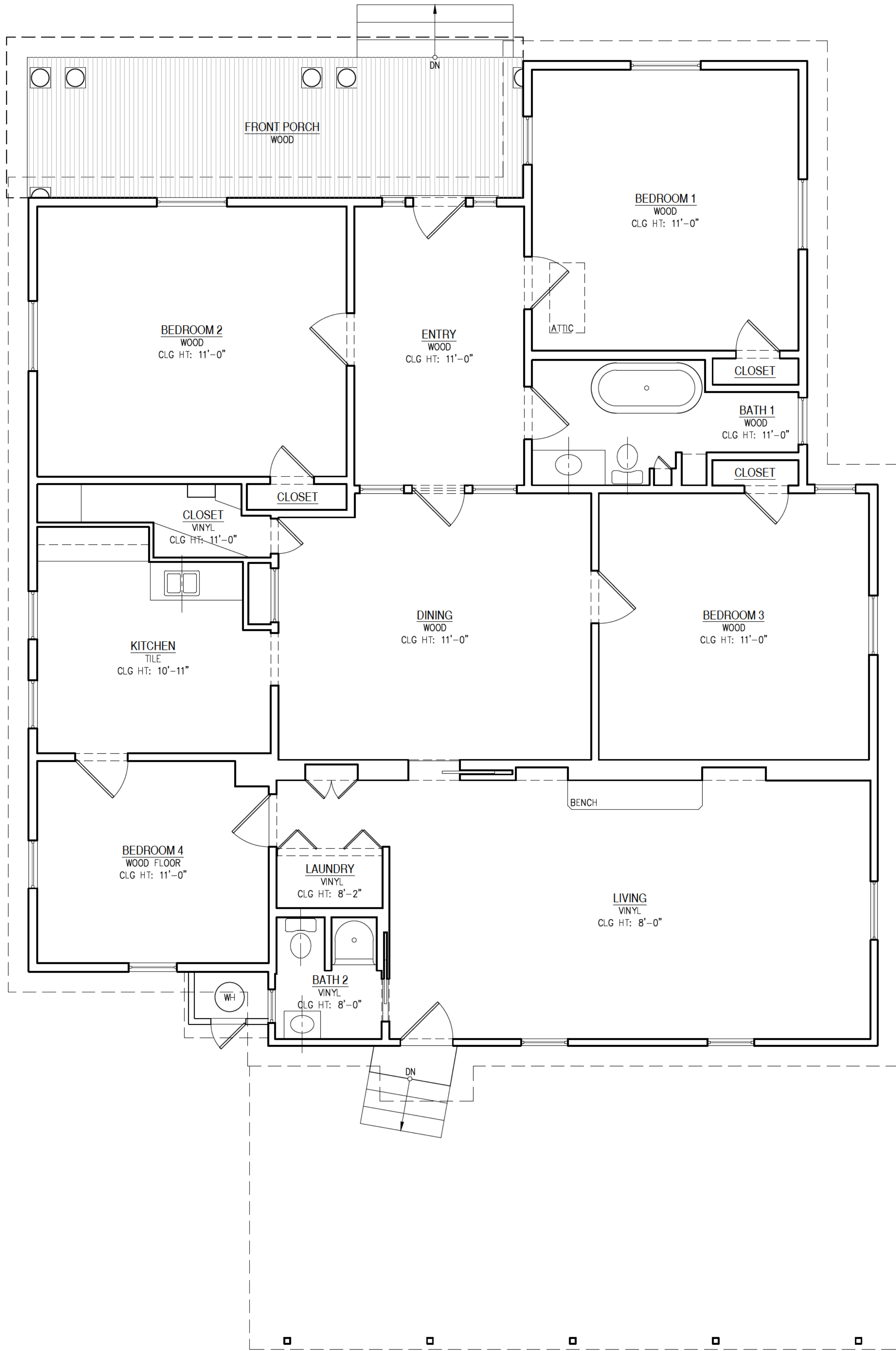
1 FLOOR PLAN: EXTG CONDITIONS SCALE: 1/4" = 1'-0"
