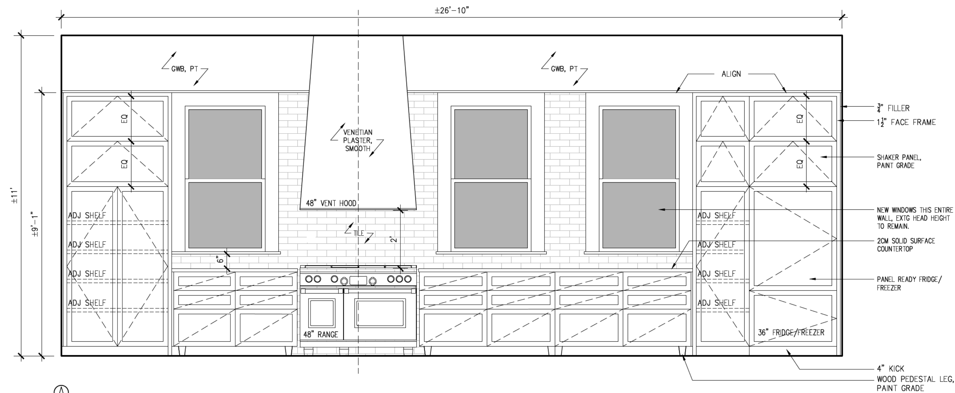
1 INTERIOR ELEVATION: KITCHEN SCALE: 1/2" = 1'-0"
